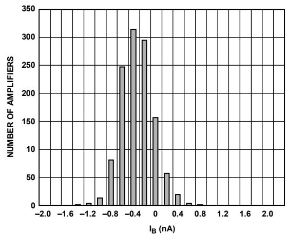
Figure 8. Input Bias Current, V_{DS} = \pm 5\text{ V}
